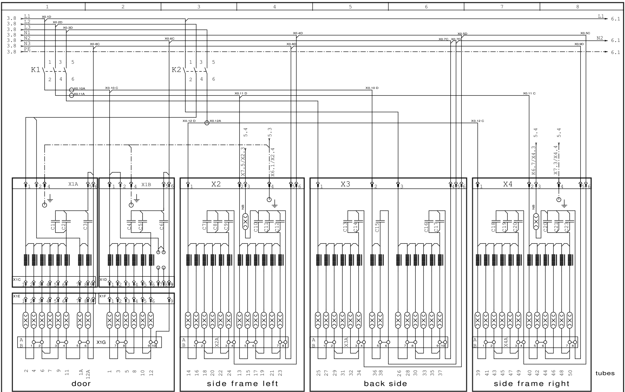
Option easy care connecting diagram (replaced page 4)
